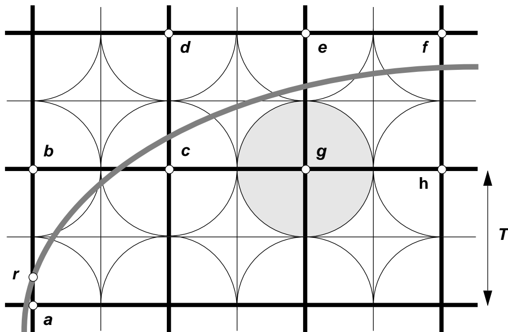
Fig. 1 Illustration of “square”, “circular” and “grid-intersect” quantization. The mesh (solid lines) has a mesh-gap T .
